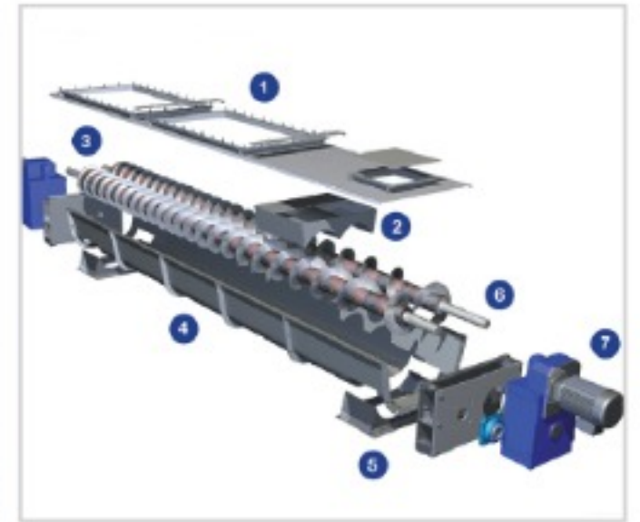
SCREW CONVEYOR
