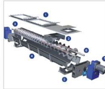
SCREW CONVEYOR
